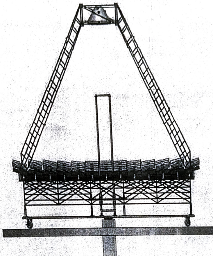
FRONT VIEW
